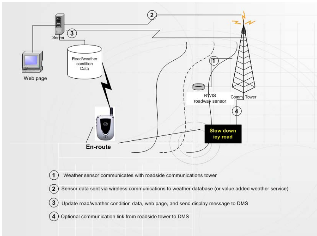
Figure 2 Typical Weather-based Travel Information System
